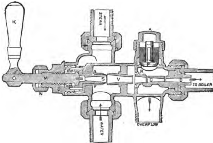
FIG. 187.—Construction of one Type of Injector. S, steam jet; V, suction jet; C-D, combining and delivery tube; R, ring or auxiliary check; P, overflow valve; O, steam plug; M, steam valve and stem; N, packing nut; K, steam valve handle; X, overflow cap.
